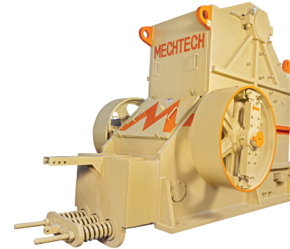
DOUBLE TOGGLE JAW CRUSHER DTJC SERIES
